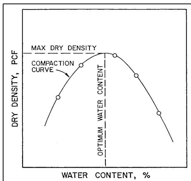
Figure 1. Compaction curve.
